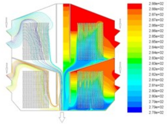
Fig. 13: Approximate two- dimensional numerical simulation of the temperature distribution
