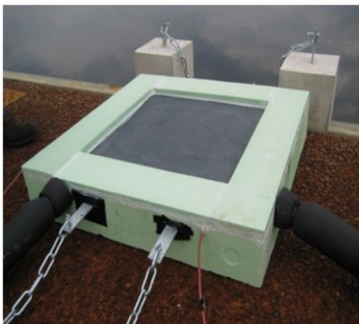
Fig. 16: Plate-shaped underwater heat exchanger with anchor and thermally insulated flow and return pipe
